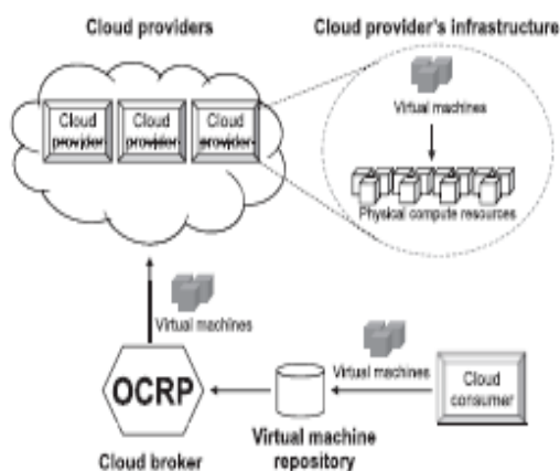
Fig. 2. System model of cloud computing environment.
